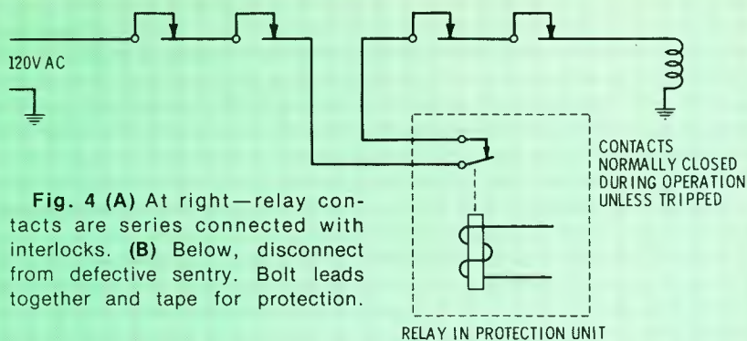
TRANSMITTER INTERLOCK CIRCUITS
