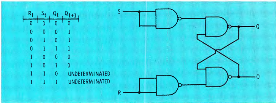
Fig. 3 R-S (Reset-Set) flip-flop. This NAND gate implementation is unlocked. The subscripts t and t + 1 now refer to the amount of time required for a change on the input to cause a change on the output. Q_{t+1} represents the output state this time interval after applying the inputs R_t and S_t .
