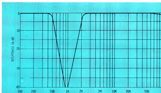
Fig. 4 Filter response curve of a high quality IM meter.
